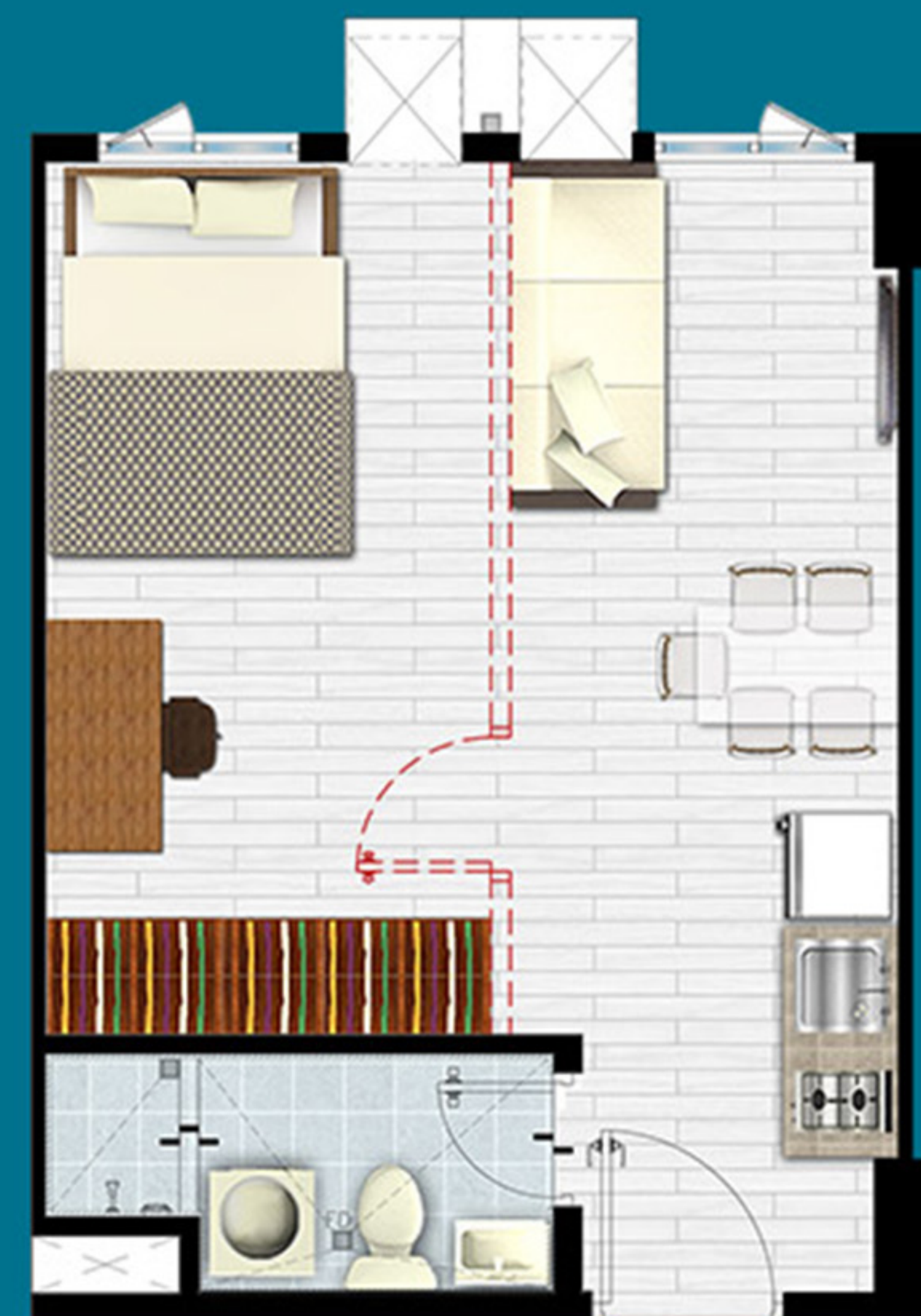
1 BEDROOM FLEXI SUITE UNIT (Suggested furniture layout) ±28.52sqm
